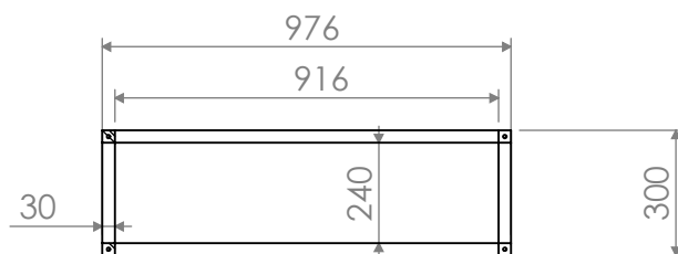
SECTION E-E SCALE 1 : 20
