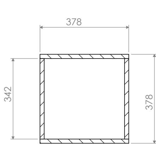
SECTION L-L
