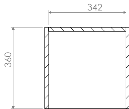
SECTION G-G
