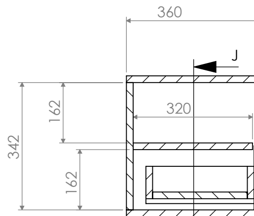
SECTION I-I
