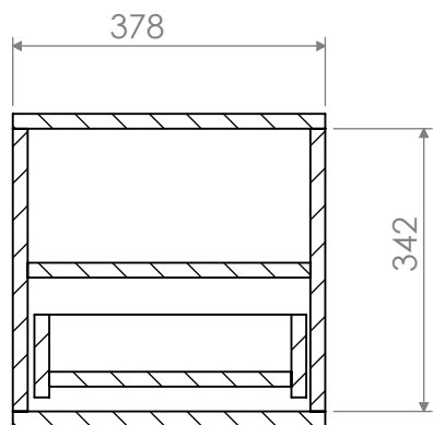
SECTION J-J
