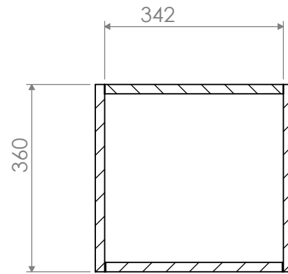
SECTION M-M
