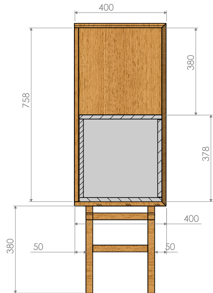
SECTION F-F
