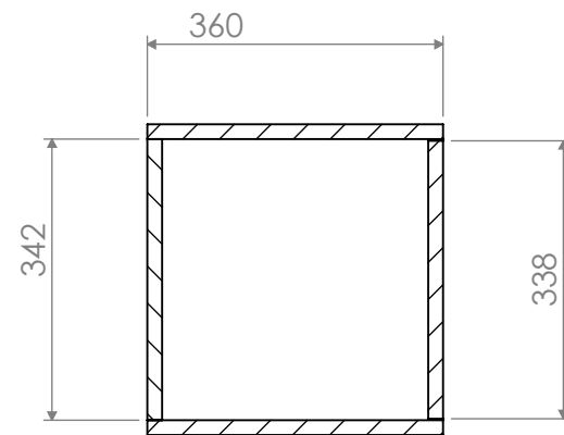
SECTION G-G
